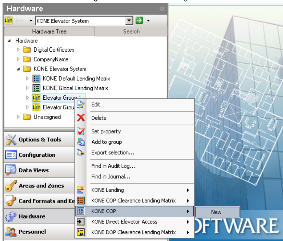
Figure 39: Access the COP Dialog Box
