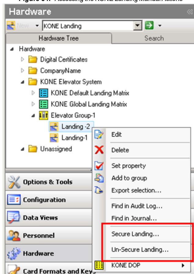
Figure 34: Accessing the KONE Landing Manual Actions
