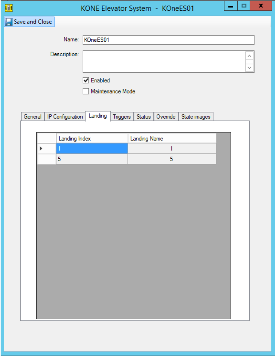
Figure 20: KONE Elevator System Editor – Landing Tab
