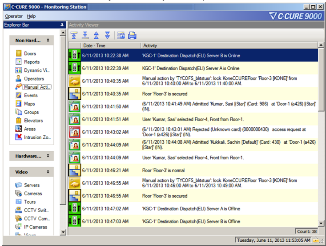
Figure 54: Monitoring Station Activity Viewer
