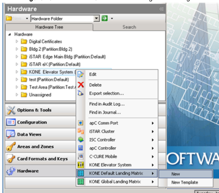
Figure 28: Access the KONE Default Landing Matrix Dialog Box
